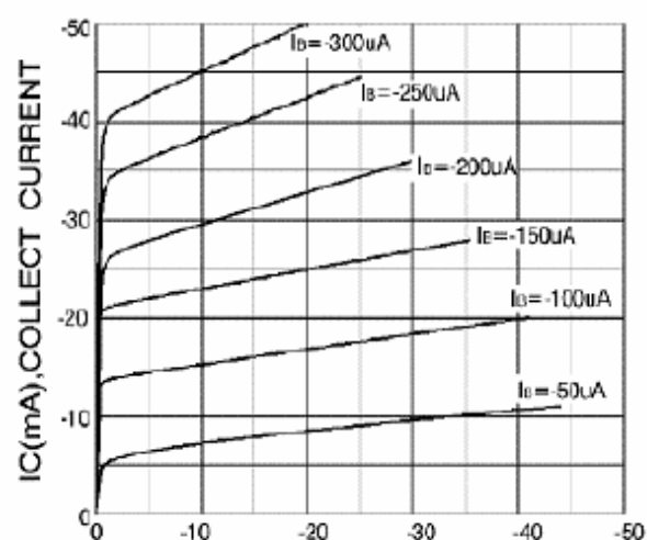
Static Characteristic
