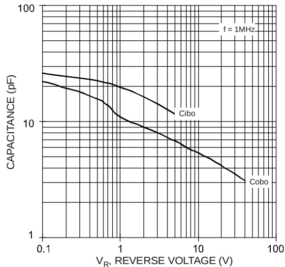
Fig. 3 Typical Capacitance
