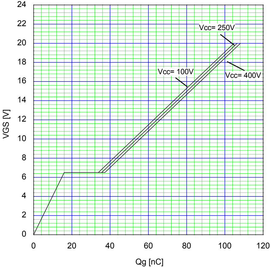
Typical Gate Charge Characteristics V_{GS}=f(Q_g):I_D=21A,T_{ch}=25^{\circ}C
