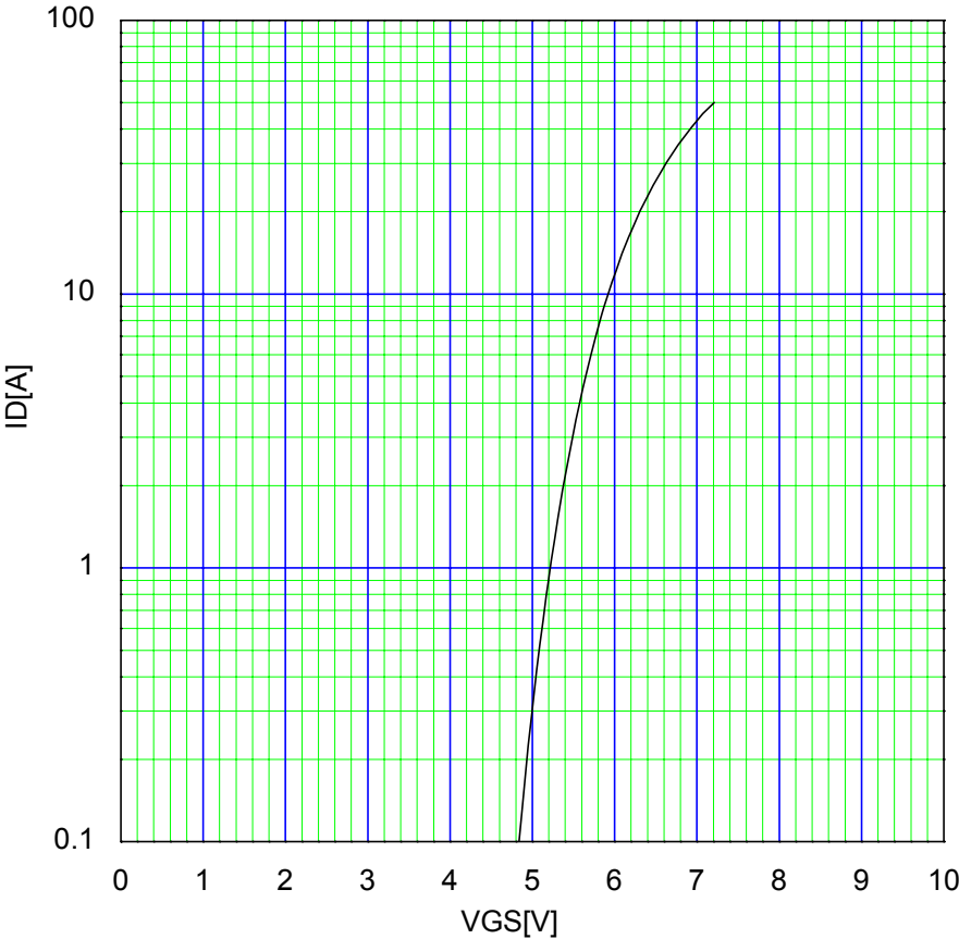
Typical Transfer Characteristic I_D=f(V_{GS}):80\text{ }\mu\text{s pulse test},V_{DS}=25\text{V},T_{ch}=25^\circ\text{C}
