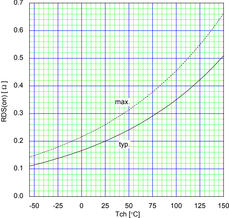
Drain-Source On-state Resistance R_{DS(on)}=f(T_{ch}) : I_D=10.5\text{A} , V_{GS}=10\text{V}
